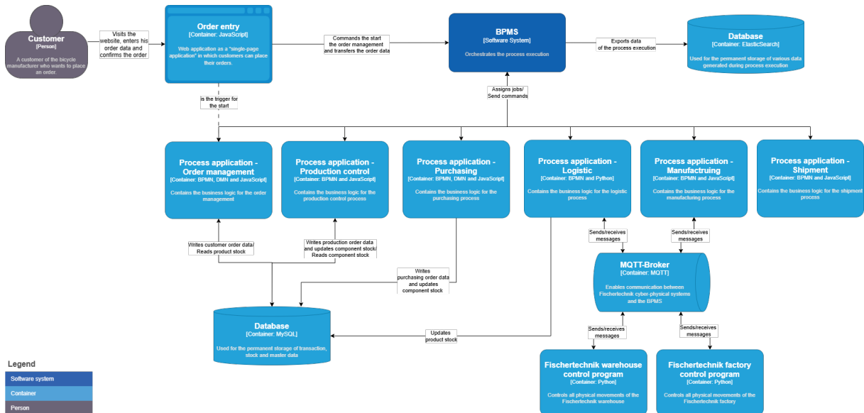
Figure 4.2.: C4 container diagram (adapted from Iyebi Itomb 2023)
