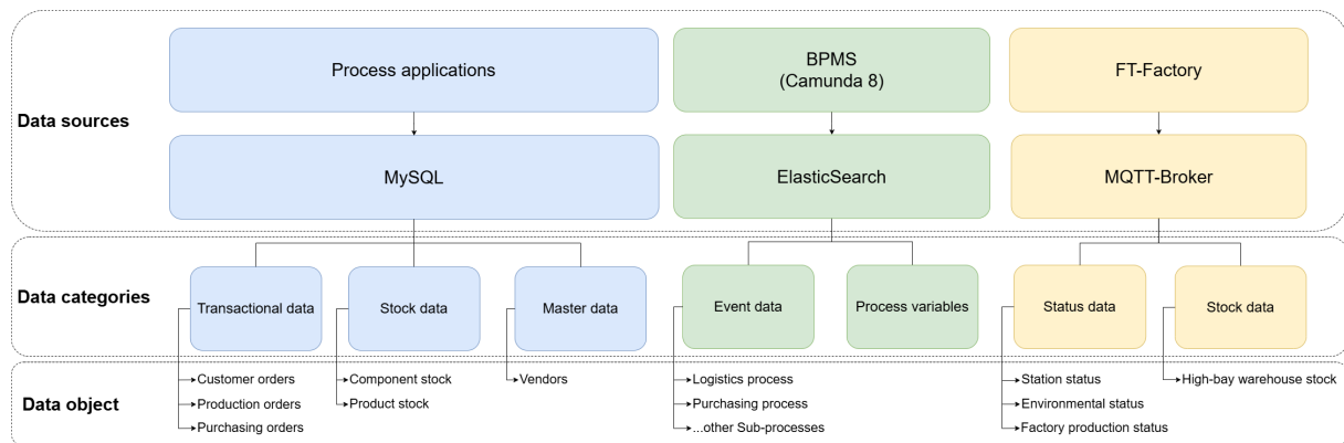
Figure 5.1.: Data overview in the BPA Lab (Gonzalez 2025)
