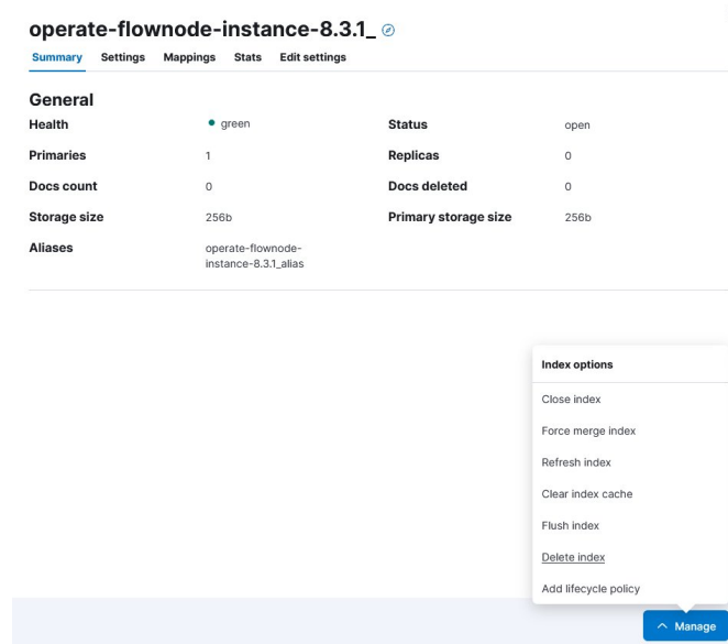
Figure 7.10.: Delete the existing operate-flownode index
